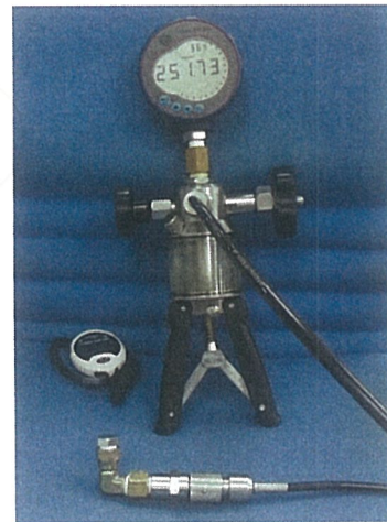
Hydrostatic Test
